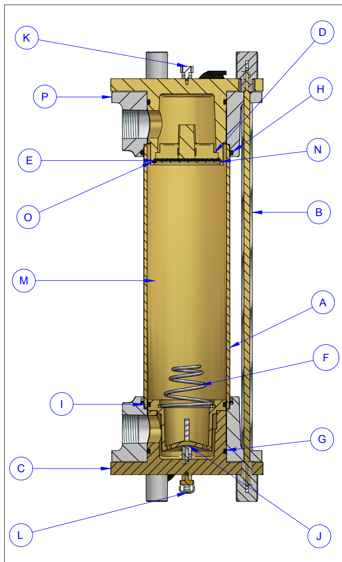
Figure 3 - FLO-DRI cross section view (same as page 5)
