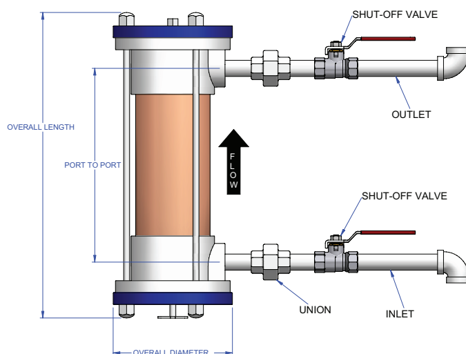
Figure 1 – G-60, G-100, G-150, M-60, M-100 & M-150 Series Assembly Diagram
