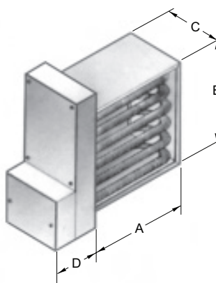
Figure 18 – Type DIF
