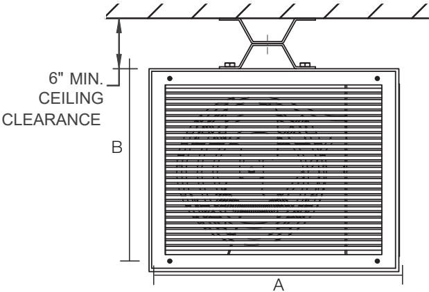
Figure 33 – Ceiling mount with clearances
