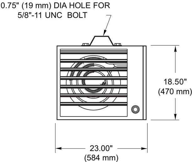
Figure 36 – Horizontal air flow ceiling mount
