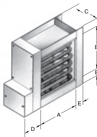
Figure 17 – Type DFF
