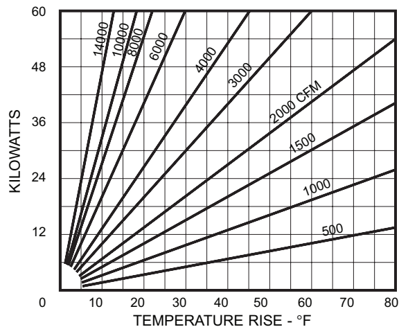
Figure 12 – Recommended Kilowatts
