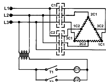
Figure 7 - Wye To Delta Transformation
