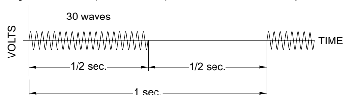
Figure 1 Fixed (one second) time base at 50% output
