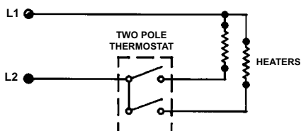
Figure 4 - Use of Contactor (Single Phase)
