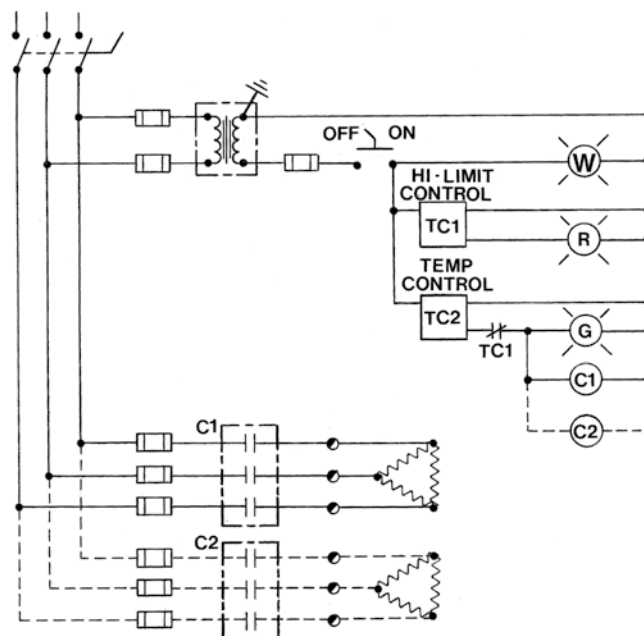
Type CPA Control Panels (Type 4 Enclosures) 208V, 240V, 480V, 600V, (1 or 3 Phase)
