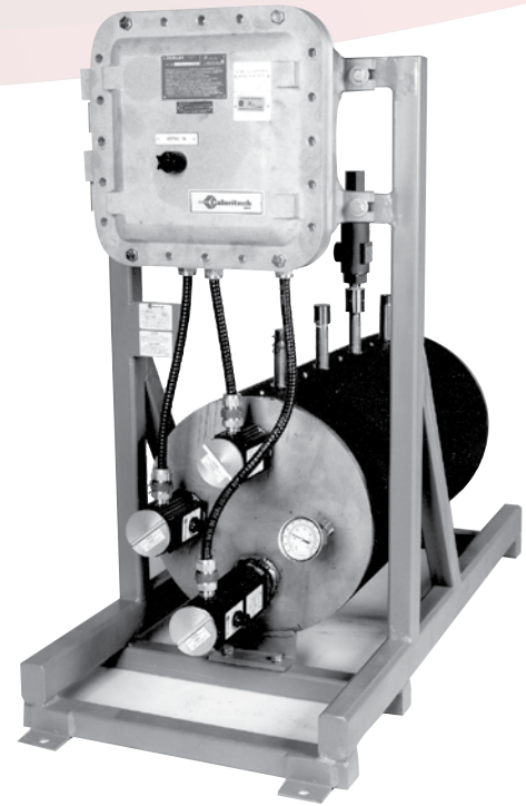
"Domestic" Water Heater For Hazardous Locations 600V 6000W
