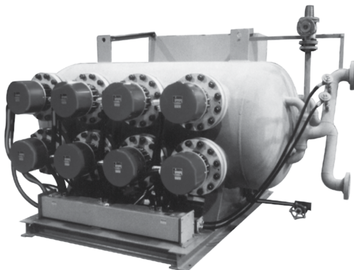
Steam Superheater 600V 324 kW 150 PSIG Operating Temperature 750°F (399°C)
