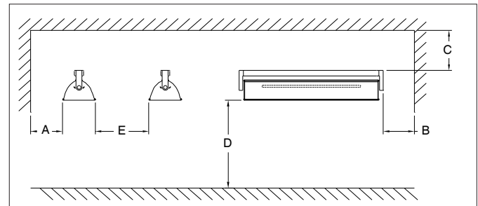
Figure 1 – Mounting Clearances
