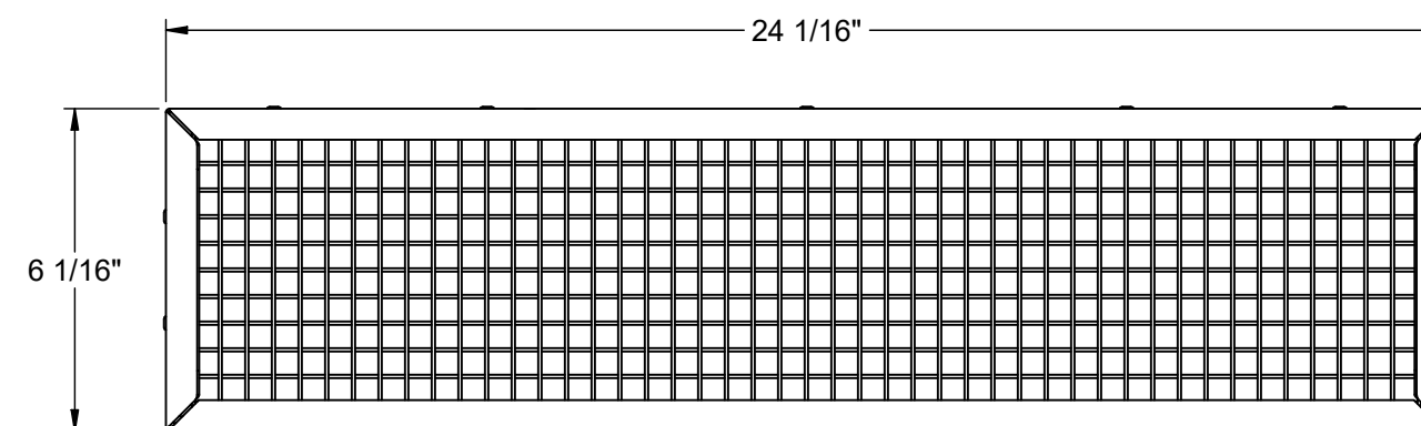
FRONT 1:4
