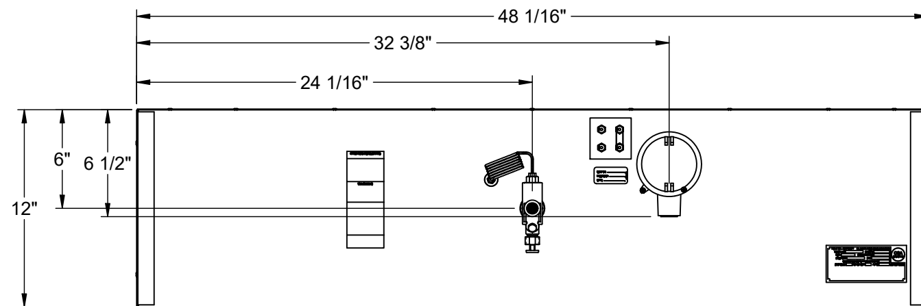
BACK 1:8
