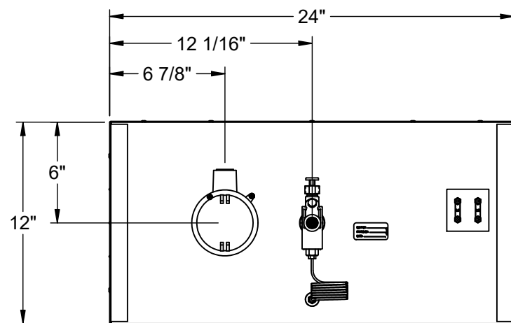
BACK 1:8
