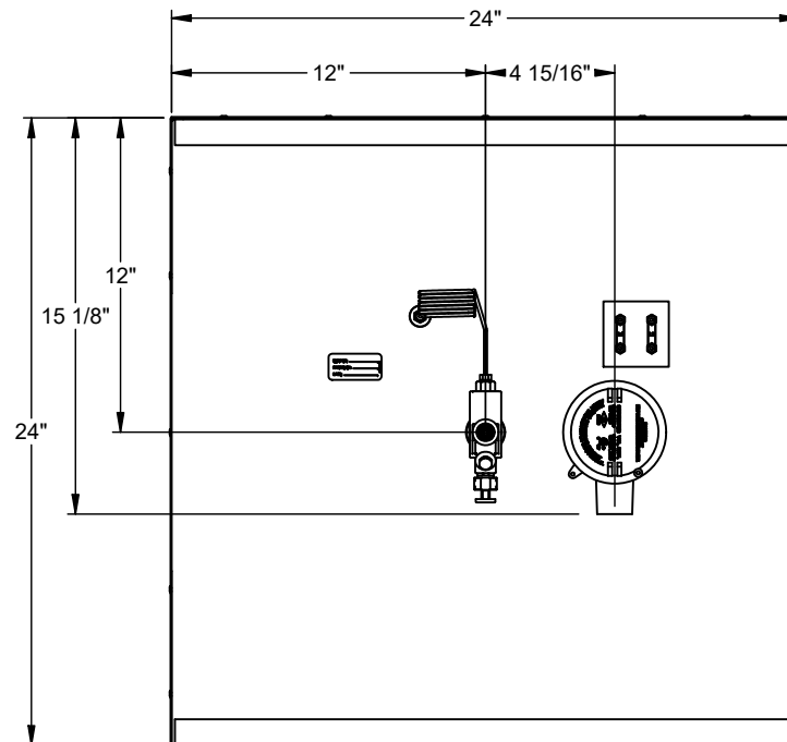
REAR 1:8
