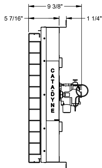
SIDE 1:10
