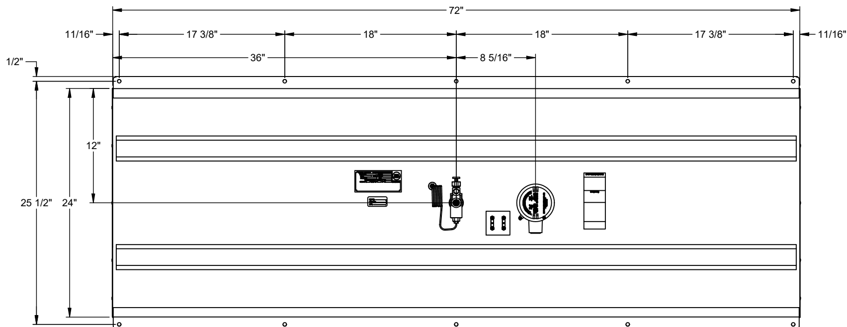
REAR 1:10
