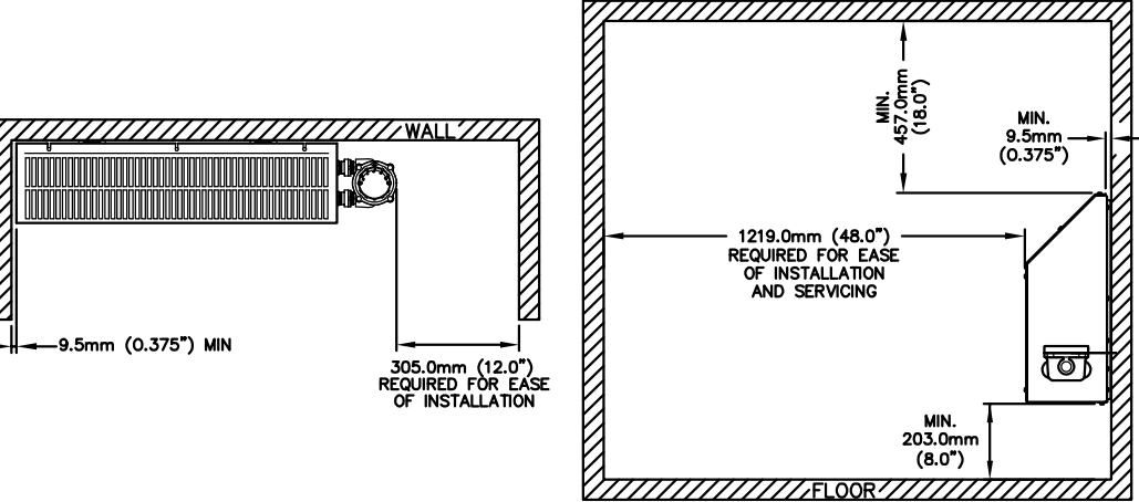
INSTALLATION CLEARANCES
