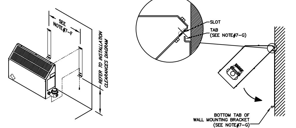
CONVECTOR MOUNTING DIAGRAMS
