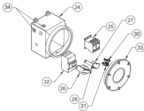
Control Enclosure
