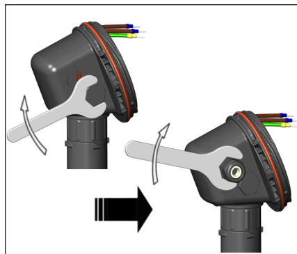
10. Install M25 power gland (order separately) and M25 blind plug. For in-line splice, T-splice, or end termination, install additional M25 blind plug (order M25-B-EXE separately) instead of M25 power gland.
