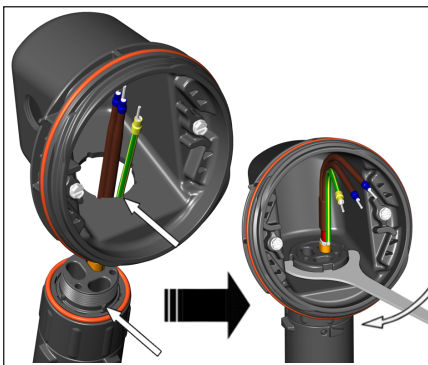
9. Mount junction box base on expediter. Make sure to align slots to properly orient junction box base. Tighten nut with Terminator-LN-Tool. If mounting horizontally, threaded gland holes must face downward.
