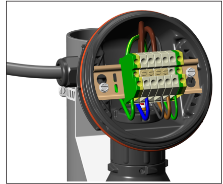
14. Complete system wiring. Terminal set screws shall be tightened to a torque value of 1.4 Nm (12.4 lb-in). See page 5 for wiring details.
