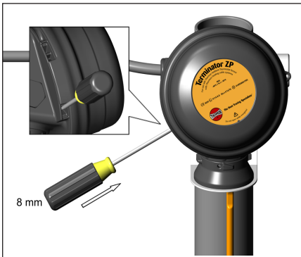
15. Install junction box lid and twist hand tight. Insert screwdriver into ratchet slots located on side of junction box base.
