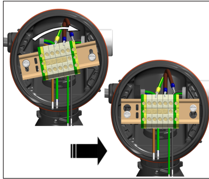
13. Install quick mount terminal blocks and tighten screws (if necessary).
