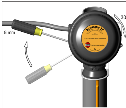
16. Use screwdriver to ratchet on junction box lid. Lid will rotate 30 degrees. To remove lid, repeat steps 15 and 16 but in the opposite direction.
