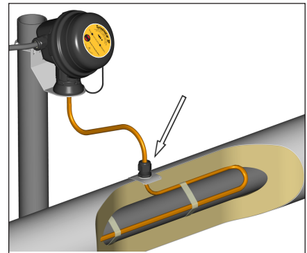
17. Install IEK insulation entry kit to seal heating cable penetration through insulation cladding.
