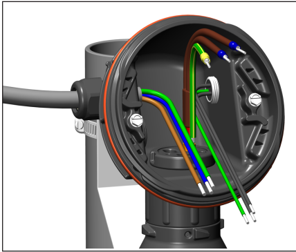
12. Install power cable.
