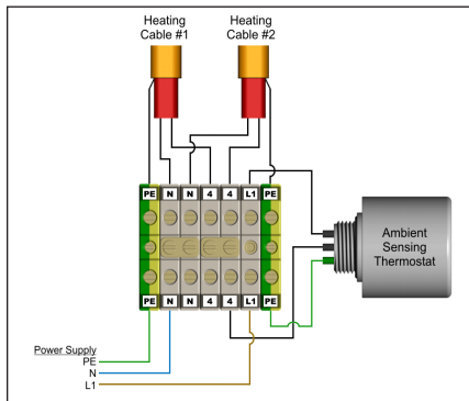
Direct Cable Switching (1 to 2 Heating Cables)
