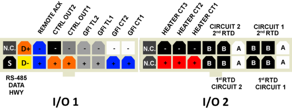
Figure 3.2: Top-Side Connections.
