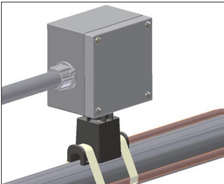
20. If using Thermon JB-K (sold separately) Install junction box lid using 4 captive screws.
