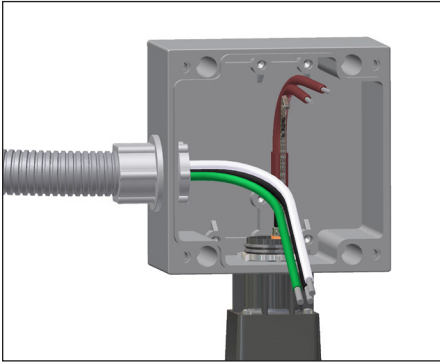
18. Install power connection fittings (supplied by others) and pull in power and ground wires.
