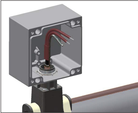
17. Mount junction box (Sold separately) on expediter using gasket and locknut provided.
