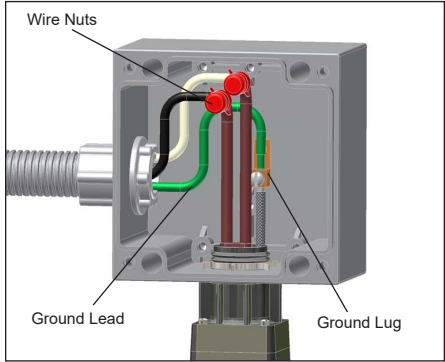
19. Complete system wiring. See typical wiring details below.
