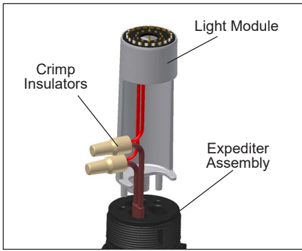
9. Snap on crimp insulators.
