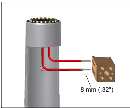
12. When using SCTK-TB Connection Kit, first trim exposed bus wires of the LED pigtail to 8 mm (.32"), then connect to the terminal block.
