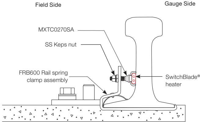
Figure 2 – SwitchBlade® Positioning
