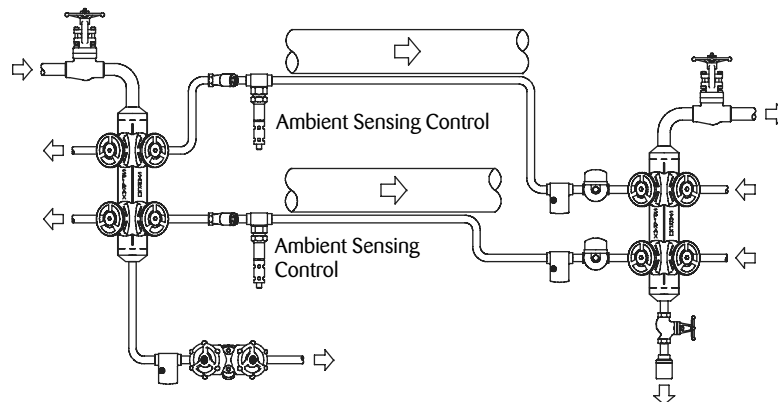
Figure 8 Tracing With Self-Acting Ambient Sensing Control
