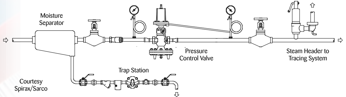
Figure 6 Steam Pressure Reducing Valve (PRV) Station
