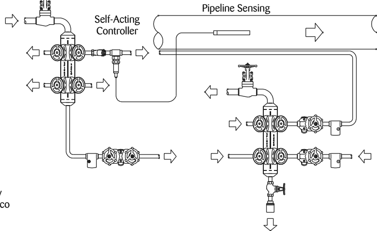
Figure 7 Tracing With Self-Acting Pipeline Sensing Control
