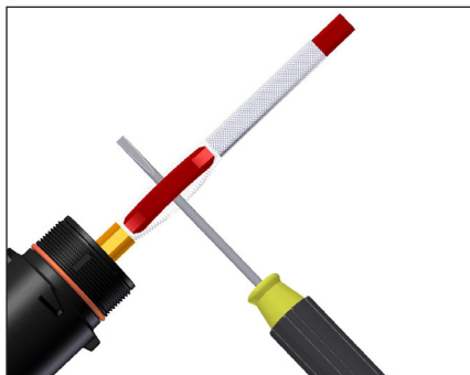
1b. Separate braid strands at edge of overjacket and pull cable through opening in braid.
