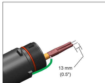
3c. Expose 13 mm (0.5") of bus wire.
