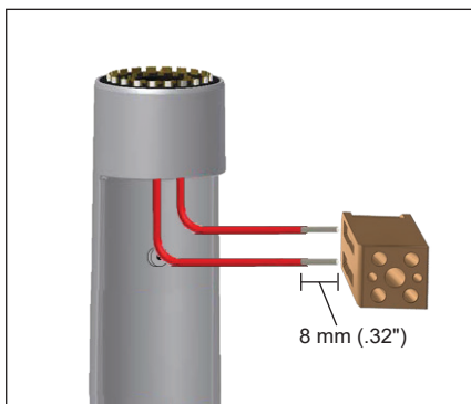
12. When using SCK-TB Connection Kit, first trim exposed bus wires of the LED pigtail to 8 mm (.32"), then connect to the terminal block.
