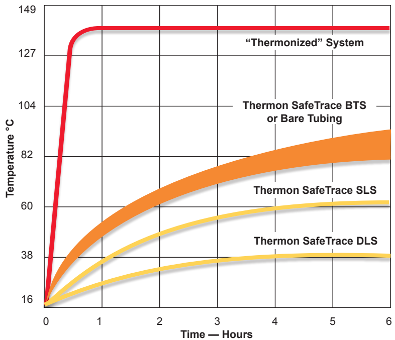
Heat-up and maintain characteristics for Thermon systems on 50mm lines with 25mm insulation with 3 barg steam service 148°C
